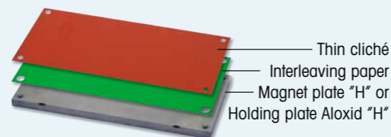
Fig.: Application example with thin cliché plate
