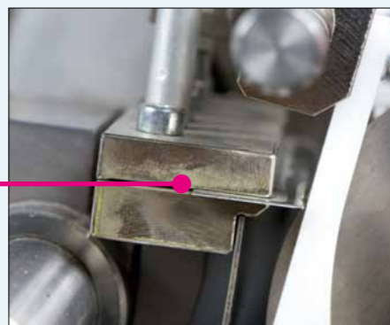
Fig.: Detailed view of rotary printing doctor blade built into doctor blade holder
